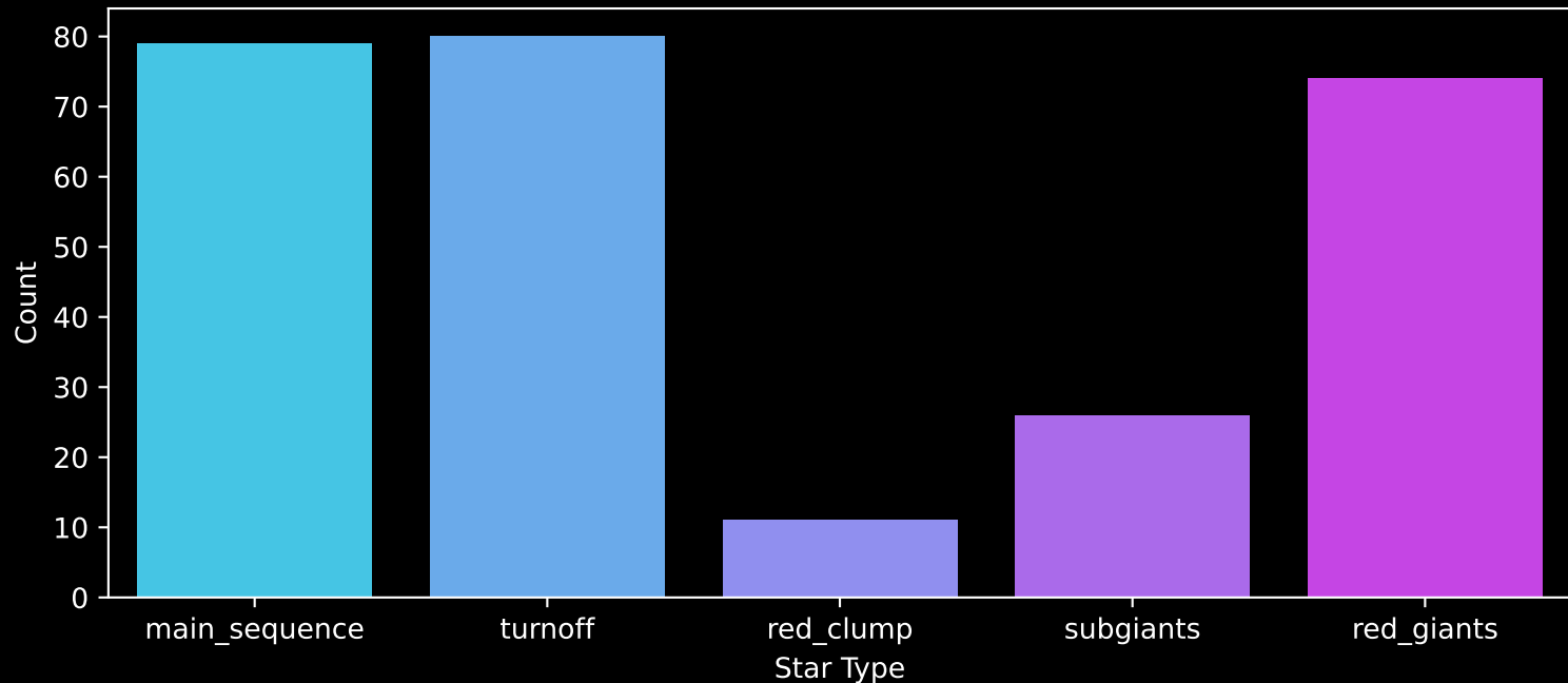
GALAH DR4 Field: [7191] Count plot of Star Type
