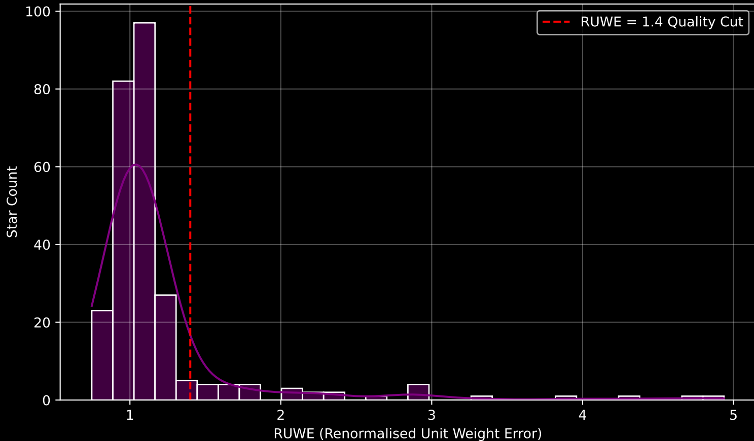
GALAH DR4 Field [7191] RUWE Distribution (n= 263)
