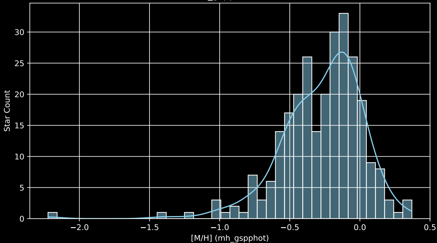
GALAH DR4 Field: [7191] [M/H] (mh_gspphot) (n= 269)
