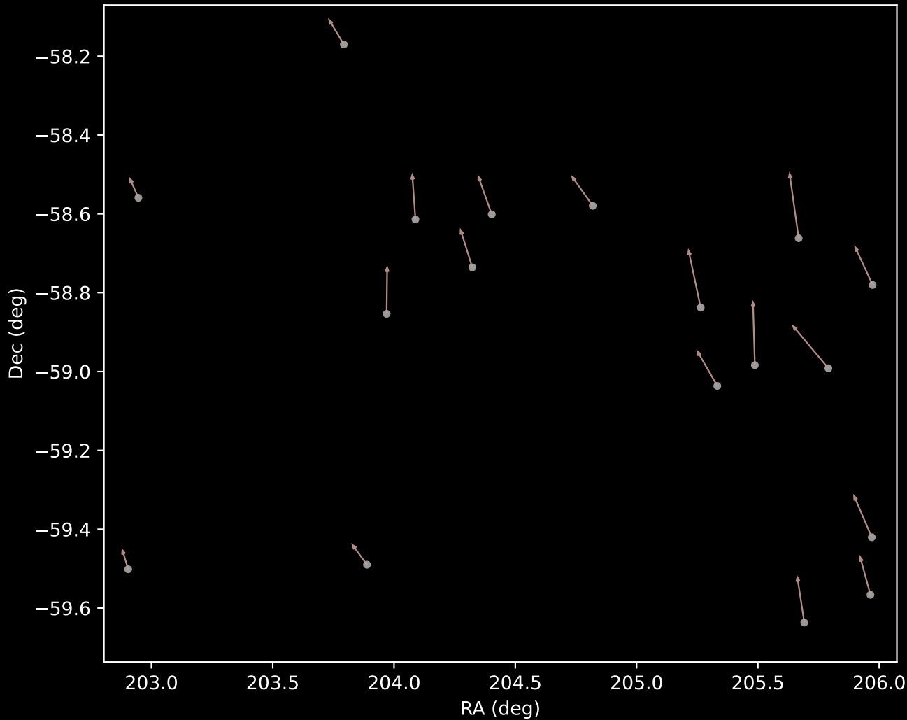
GALAH DR4 Cluster 11 Proper Motion Vectors (n=18)
