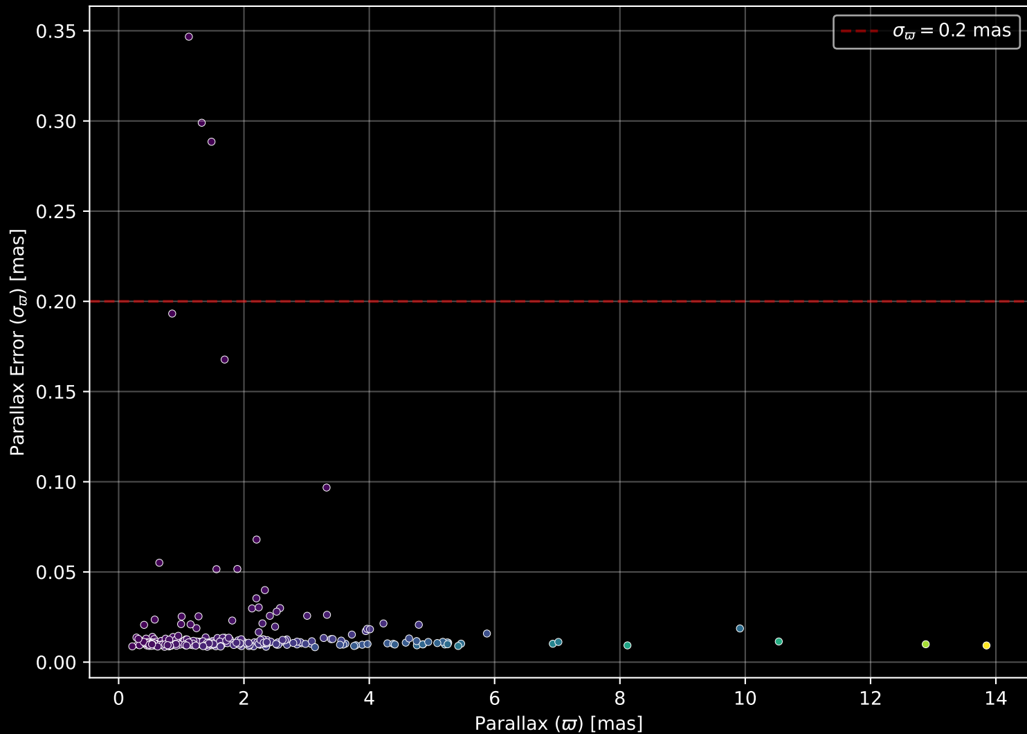
GALAH DR4 Field: [7191] Parallax Quality (n= 270)
