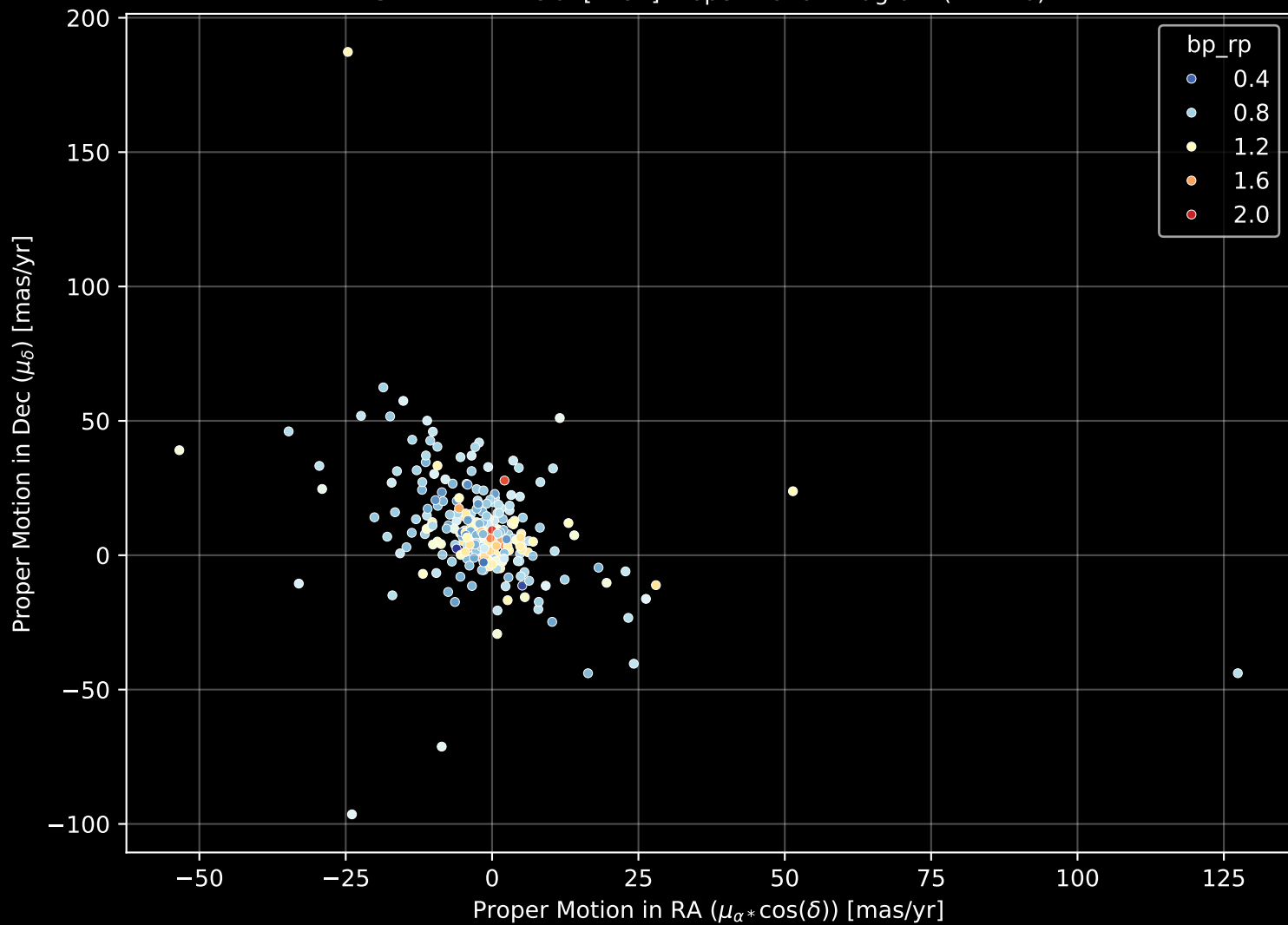
GALAH DR4 Field: [7191] Proper Motion Diagram (n= 270)
