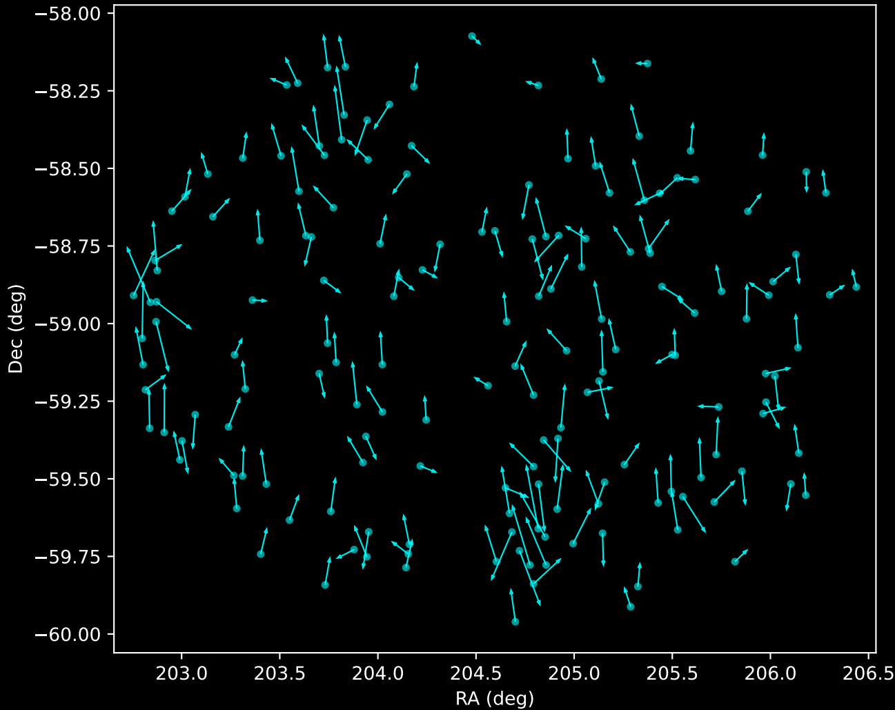
GALAH DR4 Noise Stream Proper Motion Vectors (n=166)
