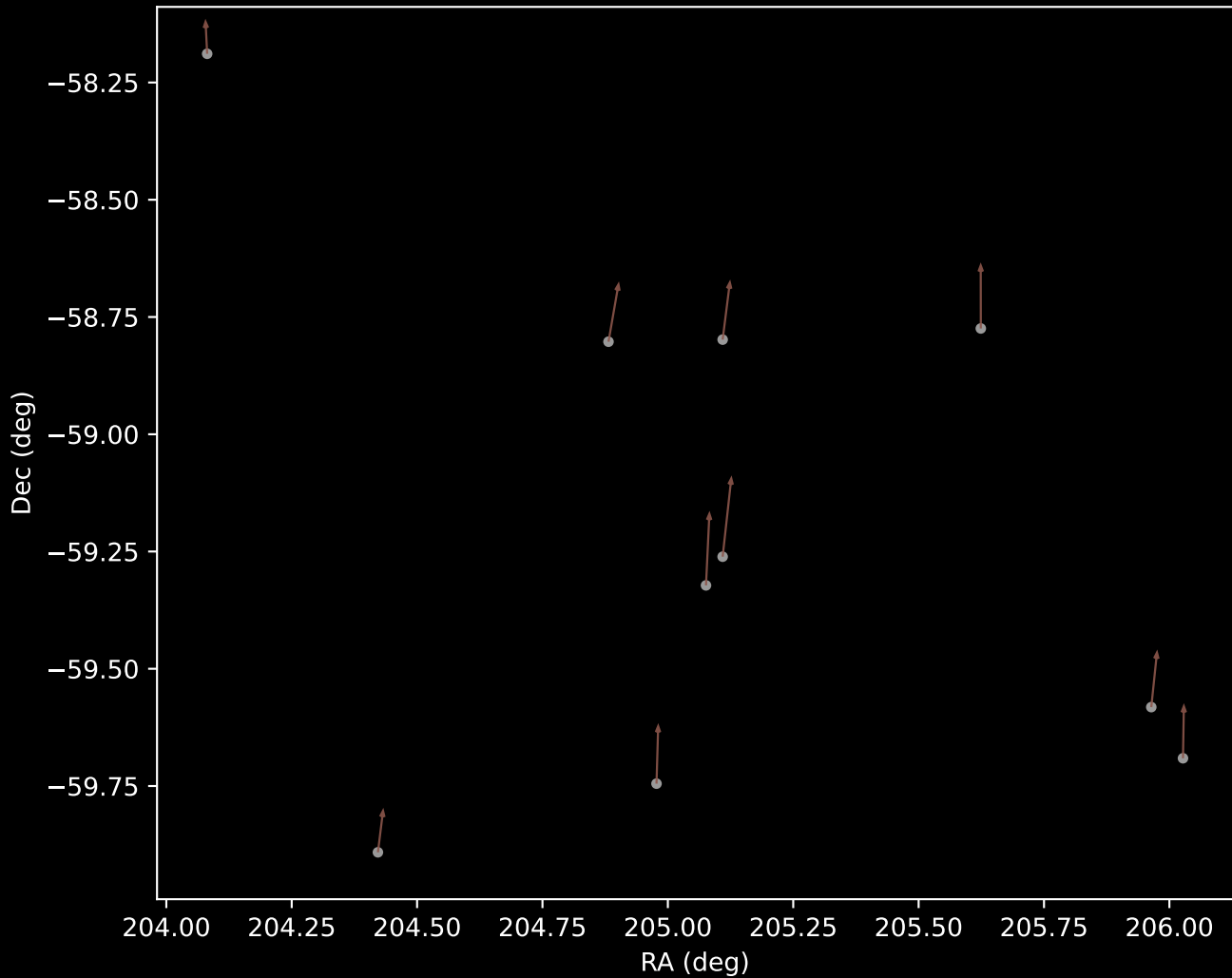
GALAH DR4 Cluster 10 Proper Motion Vectors (n=10)
